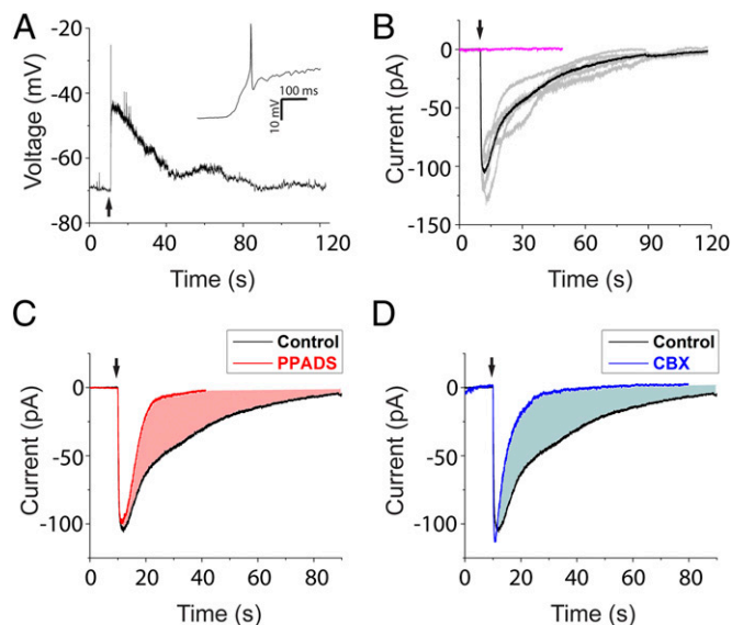
Fig. 2. ATP contributes to cell damage-induced response. (A) OHC ablation depolarized type II afferents and triggered action potentials on the rising phase ( Inset ). (B) Representative traces of damage-induced currents (at -70 mV) from five different type II afferents (gray) and the average (black). Identical needle movement that failed to ablate OHCs induced no current (magenta). (C) Average ablation-induced current in PPADS (red, three trials in three afferents) compared with average control current from B. (D) Average ablation-induced current in CBX (blue, five trials in three afferents) compared with control average.
